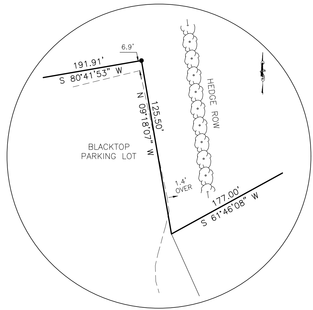
DETAIL 1"=40'
